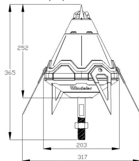
Dimensions (mm)
