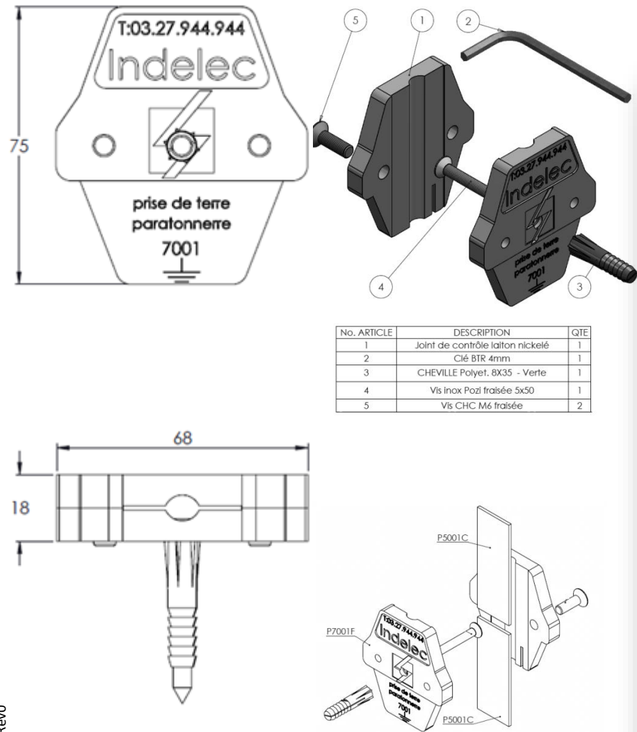
Dimensions (mm)
